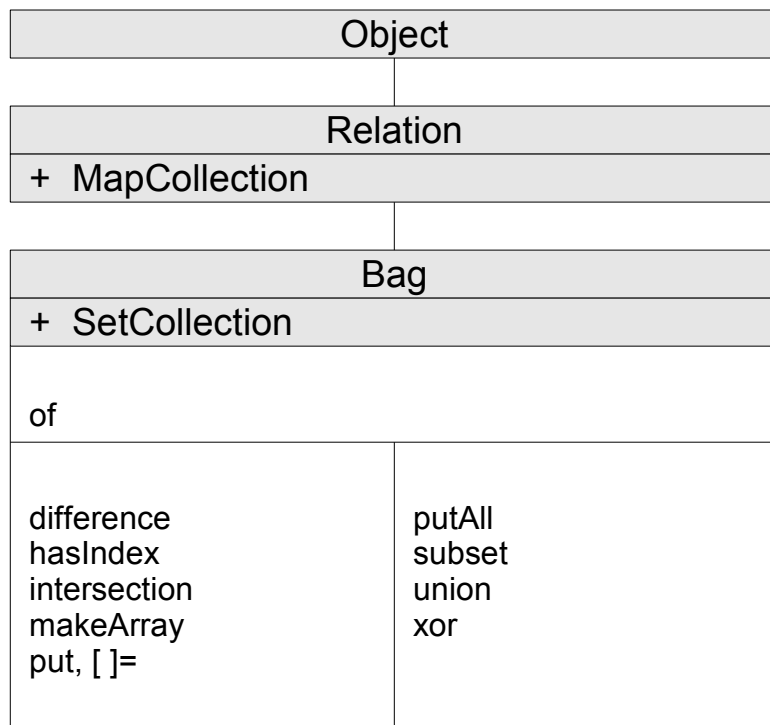
Figure 5-17. The Bag class and methods
