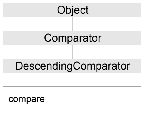
Figure 5-37. The DescendingComparator class and methods
