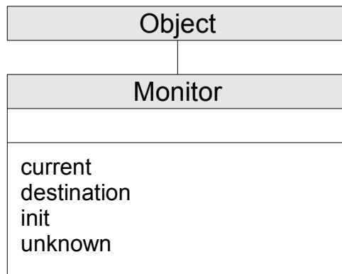
Figure 5-40. The Monitor class and methods
