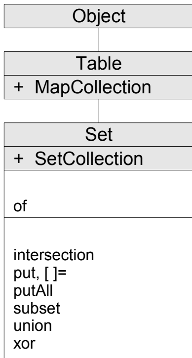
Figure 5-24. The Set class and methods
