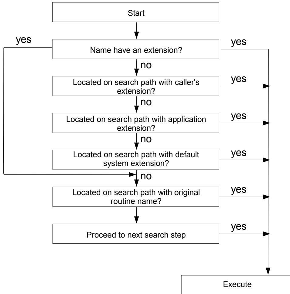
Figure 7-2. Function and Routine External File Resolution
