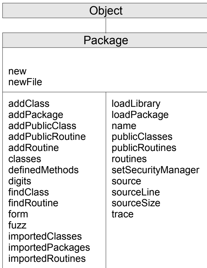
Figure 5-6. The Package class and methods
